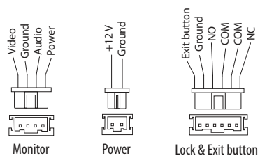
Connectors pinout
